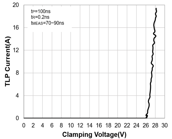
TLP Curve
